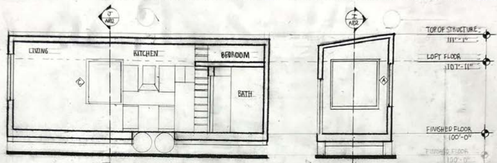
I CONG SECTION SCALE 1/4" = 1'-0"
