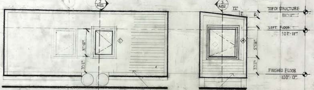
K BACK ELEVATION SCALE 1/4" = 1'-0"
