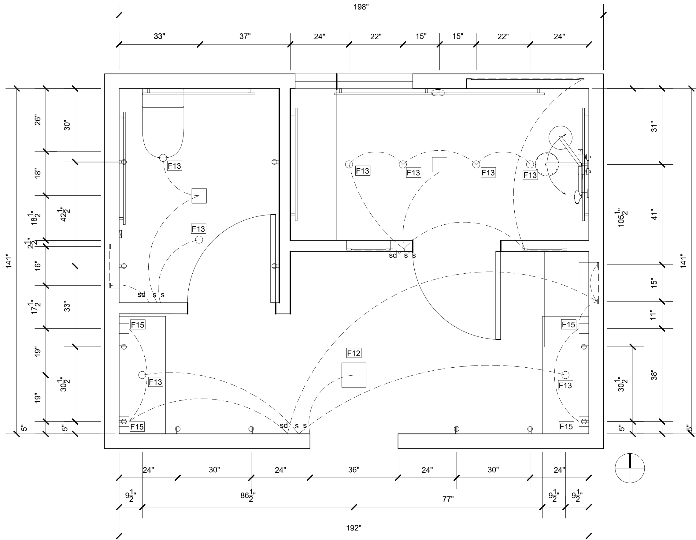
1 ELECTRICAL PLAN Scale: 1/2" = 1'-0"
